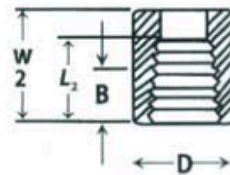
Half-Coupling
