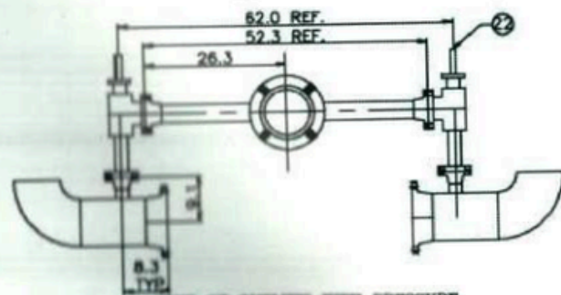
VIEW OF OUTLETS WITH PRESSURE SAFETY VALVE AND COMMON DRAIN
