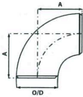
90 Deg. LR ELBOW
