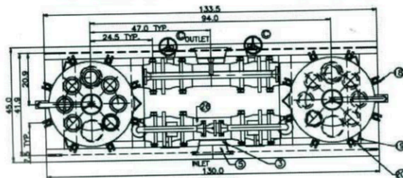
TOP VIEW SHOWN W/O TOP HEAD & DAVIT ARM ASSEMBLIES
