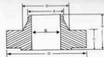
WELDING NECK
