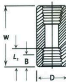
Coupling
