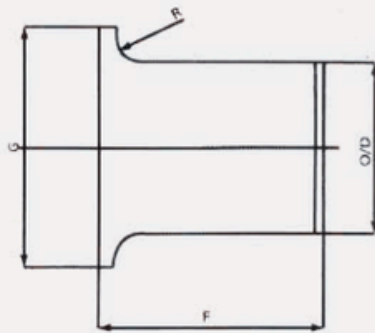
STUBEND
