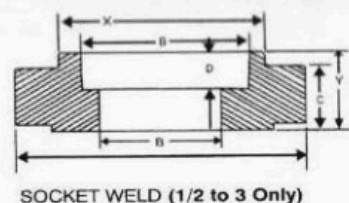
SOCKET WELD (1/2 to 3 Only)
