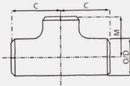
UNEQUAL TEE.
