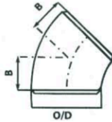
45 Deg. LR ELBOW
